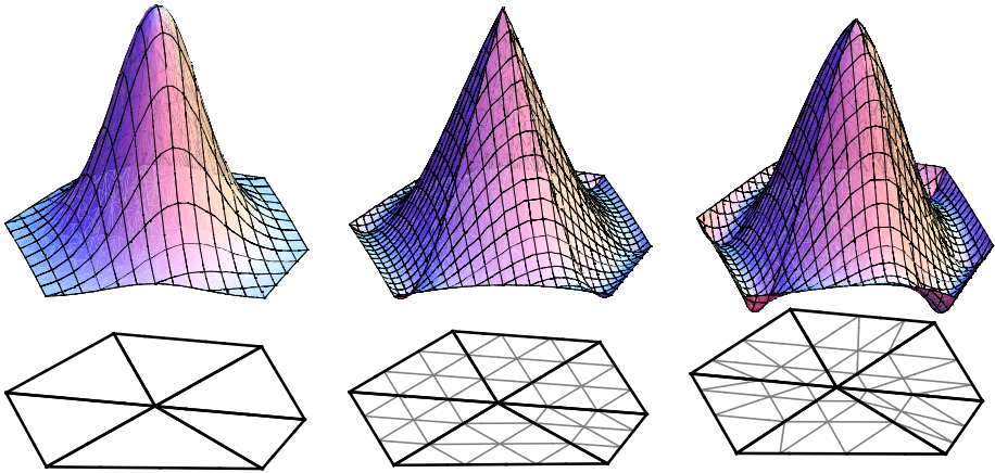
Fig. 3 The surface (14) over a star [5] with two different continuous piecewise polynomial interpolants
