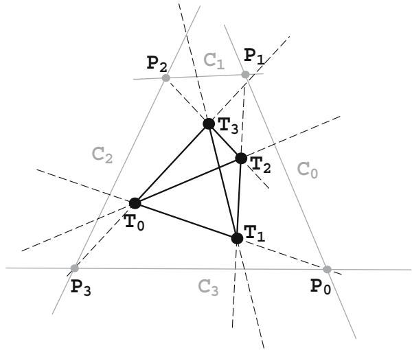
Fig. 1 A 3-simplex \langle \mathbf{T}_0, \mathbf{T}_1, \mathbf{T}_2, \mathbf{T}_3 \rangle in \mathbb{R}^3 , lattice control points \mathbf{P}_i and centers \mathbf{C}_i
