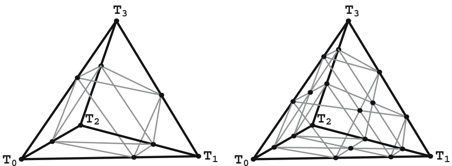
Fig. 2 The 4-pencil lattices of order n = 2, 3 on a simplex \Delta and the intersections of hyperplanes through the centers of the lattice with facets of \Delta
